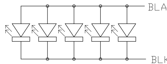
Backlight Circuit (No. of LEDs = 5pcs) Scale=free
