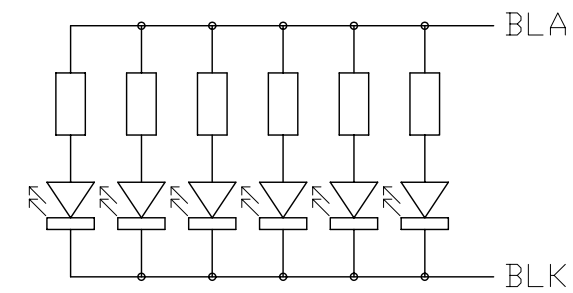
Backlight Circuit (No. of LEDs = 6pcs) Scale=free
