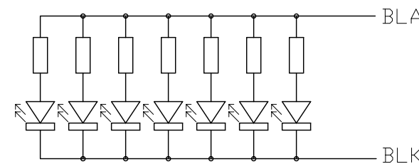
Backlight Circuit Details (No. of LED = 7pcs) Scale=free
