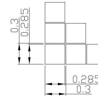
Pixels Details Scale=30/1
