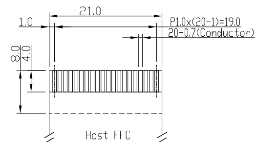
Conductor Side Details Scale=2/1
