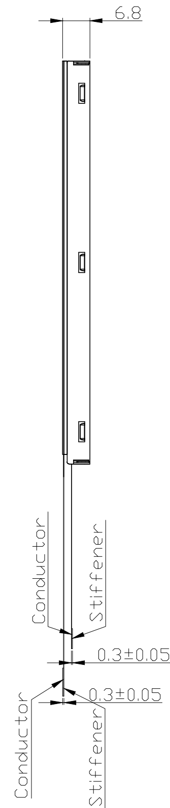
Touch Panel Logic Details Scale=free
