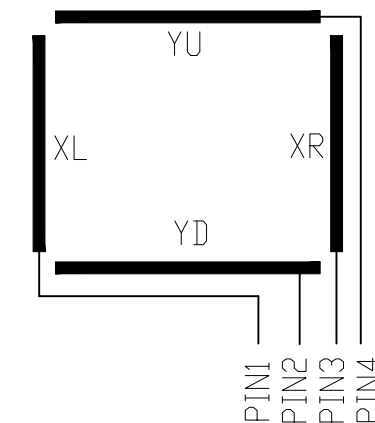
Touch Panel Logic Details Scale=free
