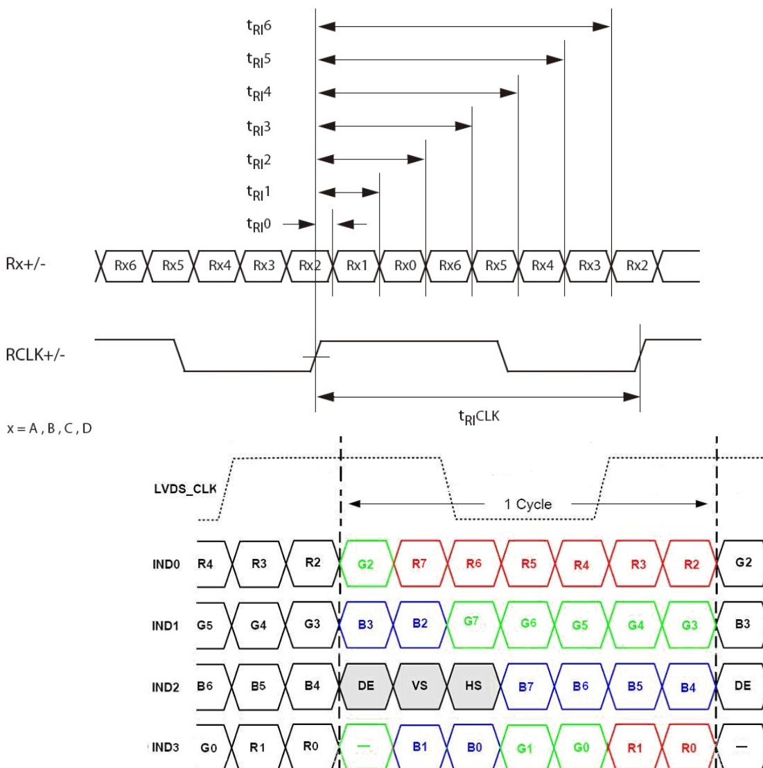
Input Clock and Data timing Diagram:
