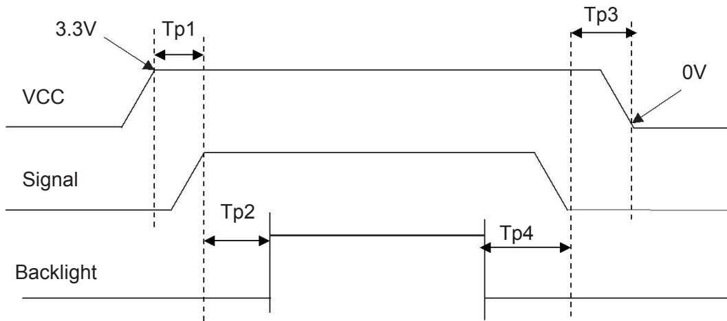
Figure5.4 Interface power on/off sequence
