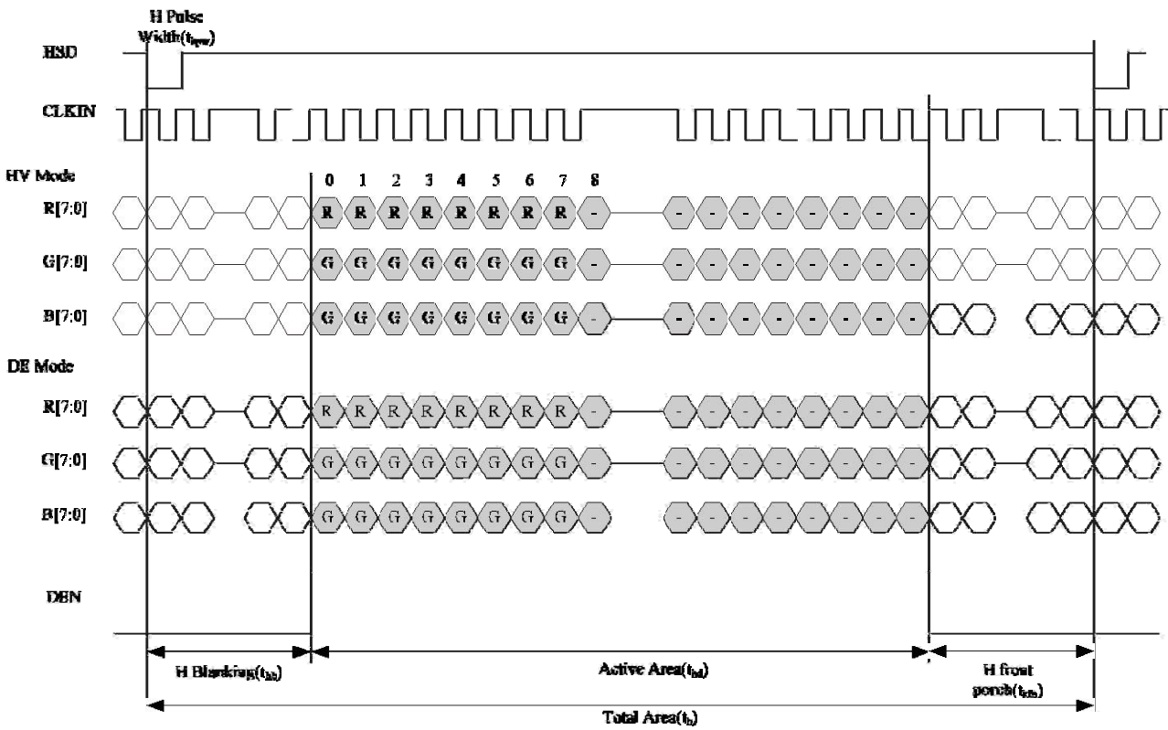
Figure 5.3.2 Horizontal Input Timing Diagram
