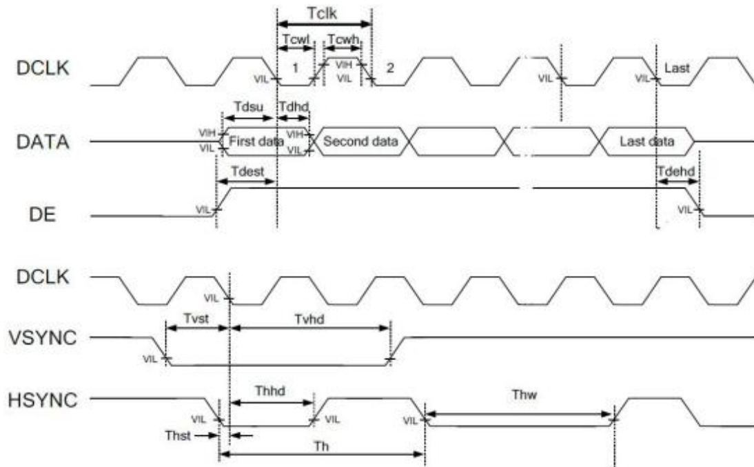
Timing Diagram
