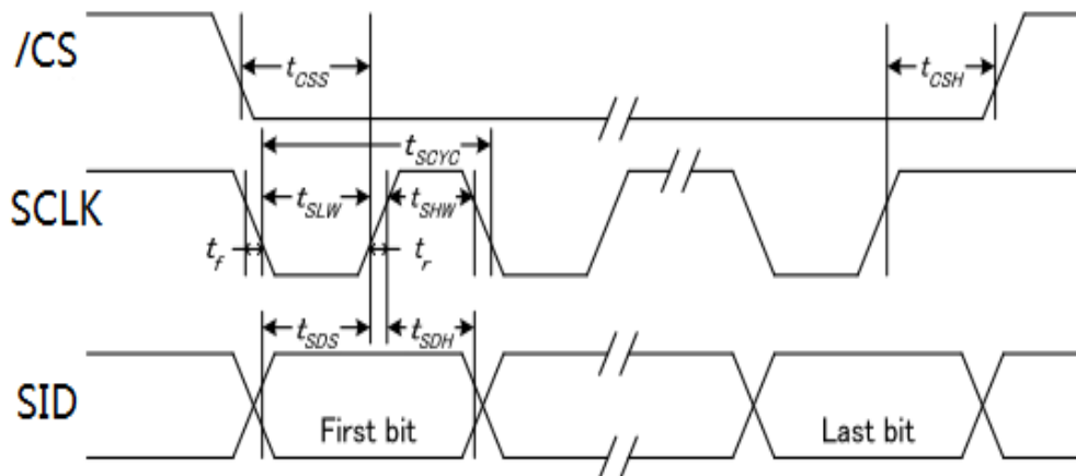
3-Line SPI Interface Timing Diagram
