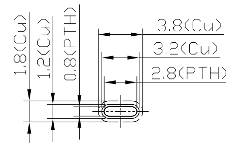
BLA/BLK Details Scale=3/1
