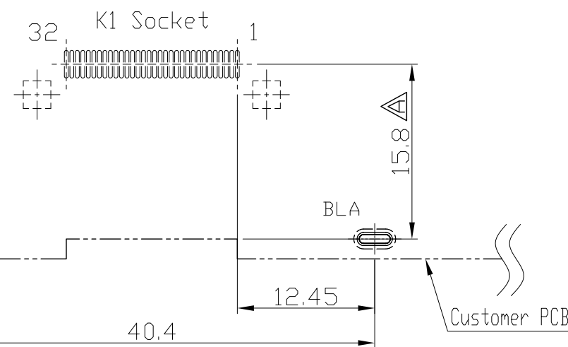
Application PCB Example (PCB Thickness=1.6t, PCB Tol=±0.15mm) Scale=2/1
