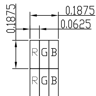
Pixel Detail Scale 50:1
