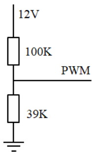
PWM circuit on LCM
