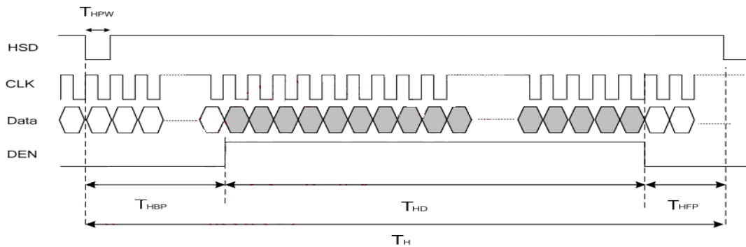
Figure 5.2 Input signal data timing
