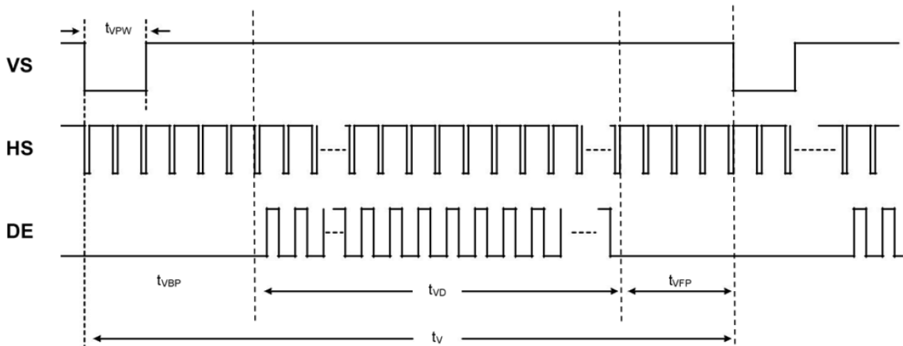
Figure 6.2 Input signal data timing
