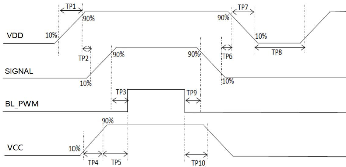
Interface Power On/Off Sequence
