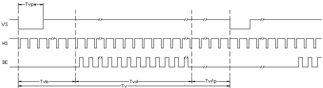
Figure 7-4-2 Vertical input timing diagram.
