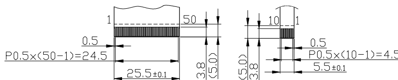
K1 Details Scale=1/1
